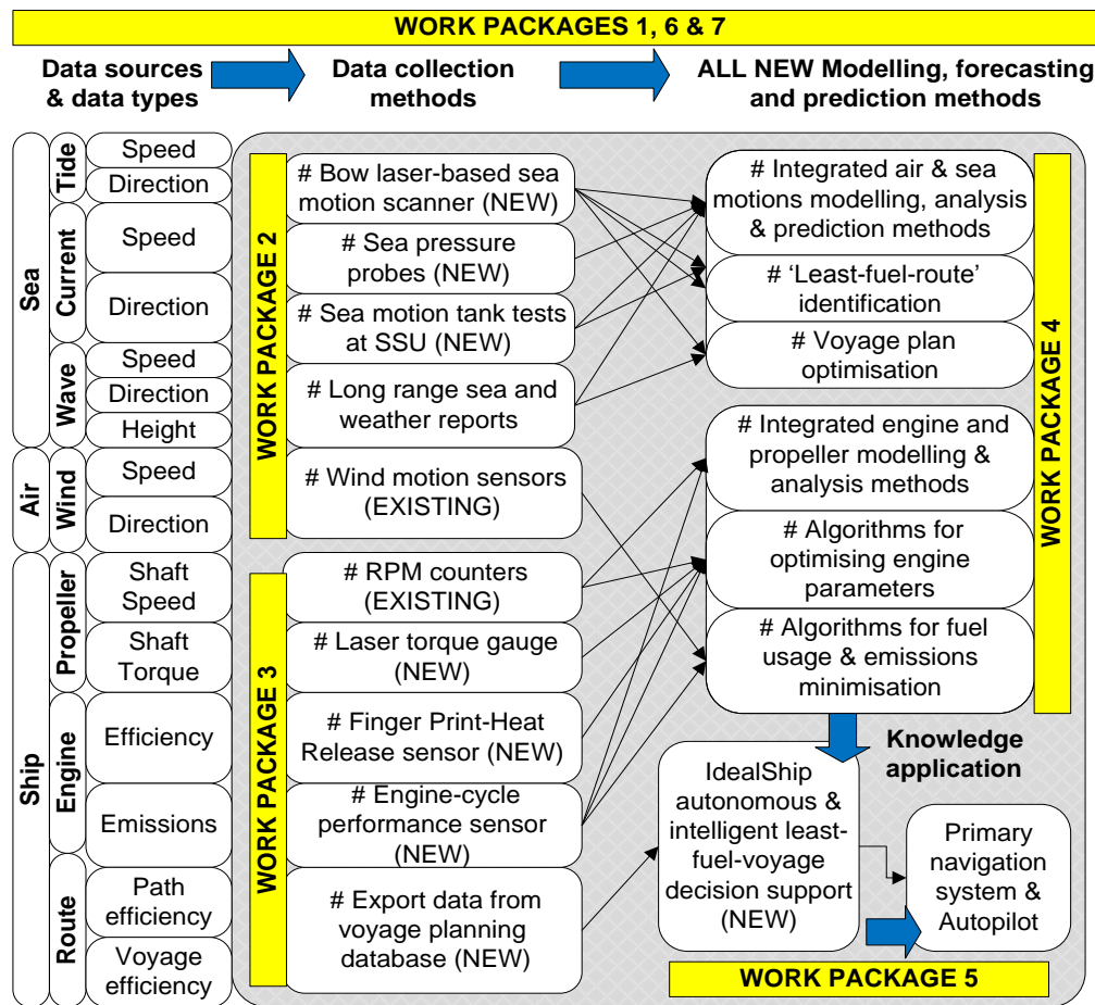
Figure 4. AutoSet System and data flow diagram
